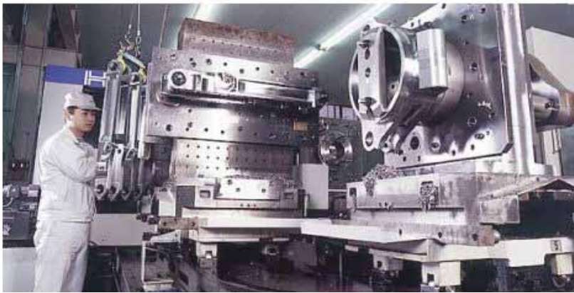
Precision machining of the large part (High tension steel)
